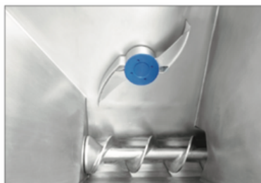
Hopper of SG 200 with feeding wing
